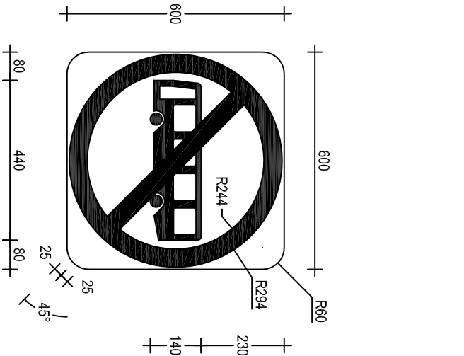
G9-87-1(A) 600 x 600
